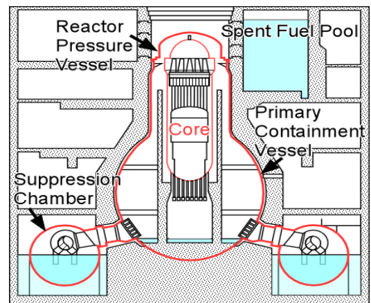
Figure 1. Cross section of BWR
