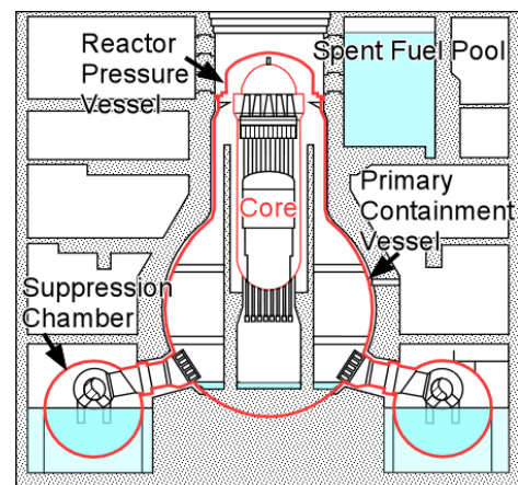
Figure 1. Cross section of BWR
